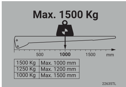
Loading diagram
