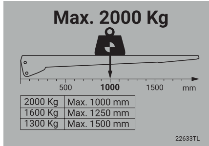
Loading diagram
