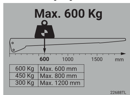
Loading diagram
