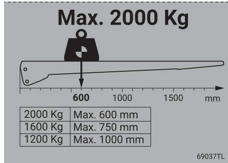
Loading diagram
