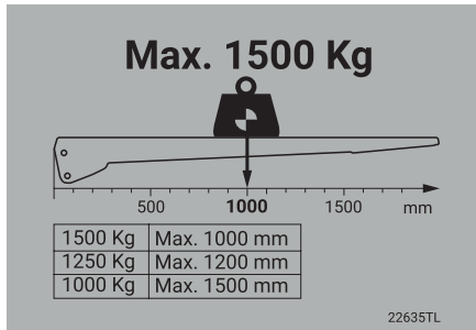
Loading diagram
