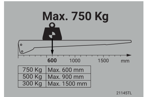
Loading diagram
