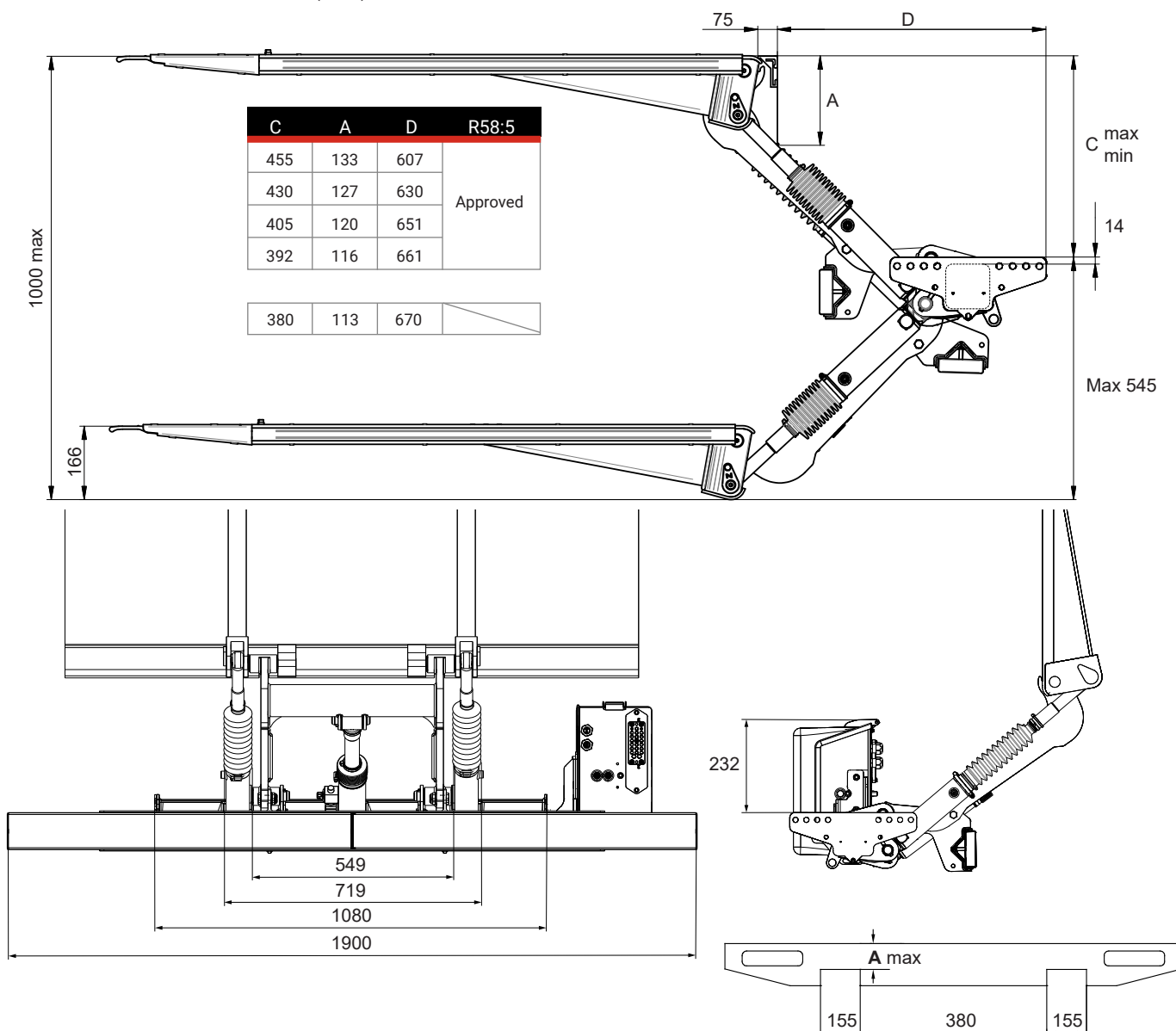
Installation dimensions (mm)
