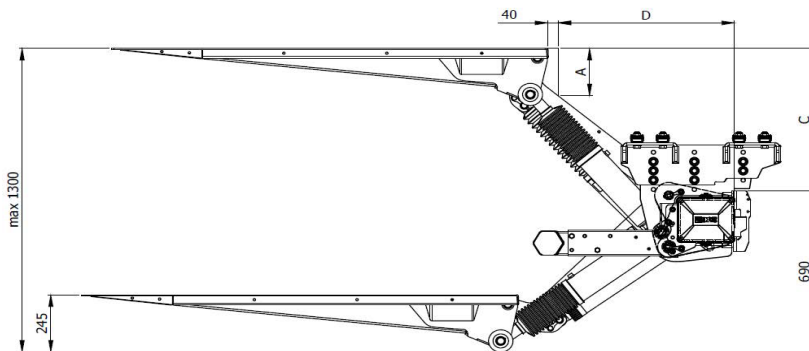
Installation dimensions (mm)
