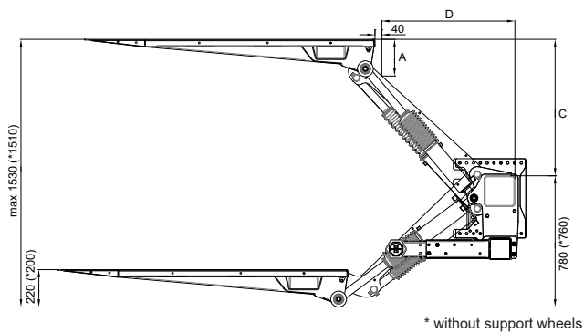
Installation dimensions (mm)
